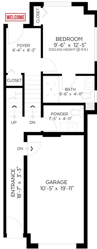
Lower Floor Plan Floor Area: 478 sq.ft. Ceiling Height: 7'-6" unless noted
