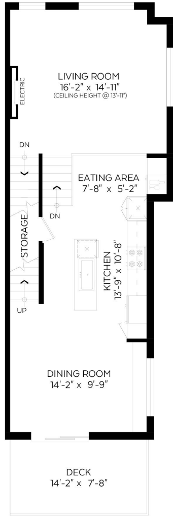
Main Floor Plan Floor Area: 735 sq.ft. Ceiling Height: 9 ft. unless noted
