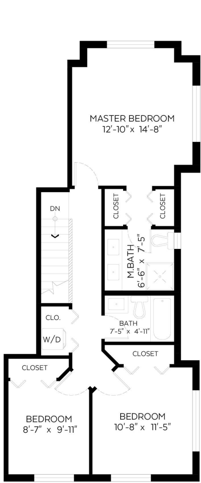
Upper Floor Plan Floor Area: 767 sq.ft. Ceiling Height: 8 ft.
