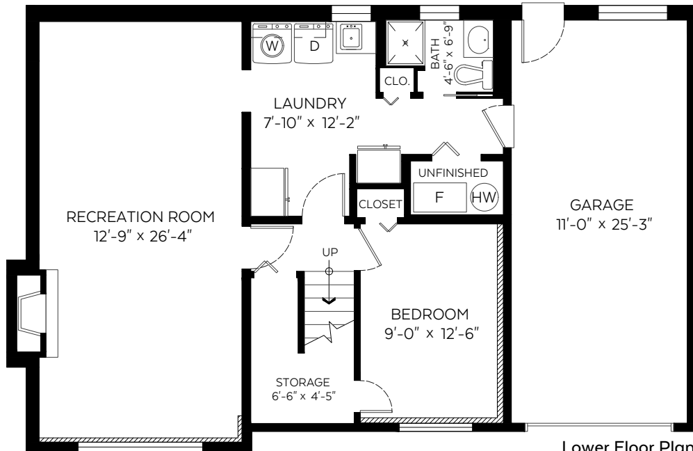
Lower Floor Plan Floor Area: 831 sq.ft.
