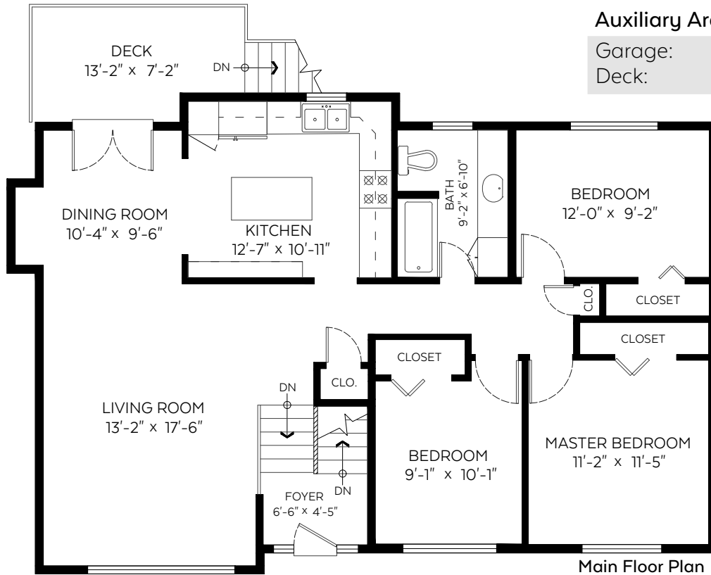
Main Floor Plan Floor Area: 1181 sq.ft
