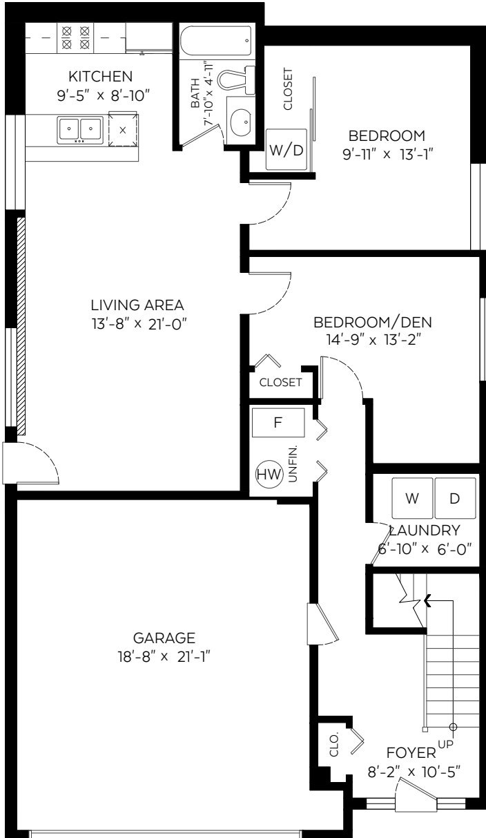
Lower Floor Plan Floor Area: 1,177 sq.ft
