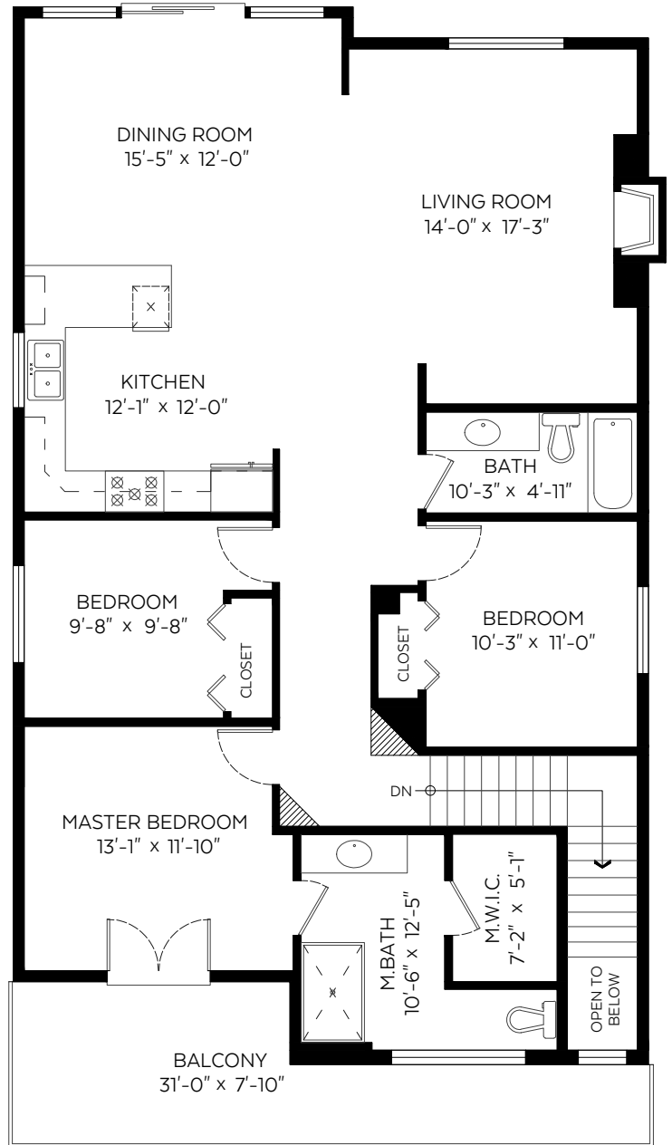
Main Floor Plan Floor Area: 1,487 sq.ft
