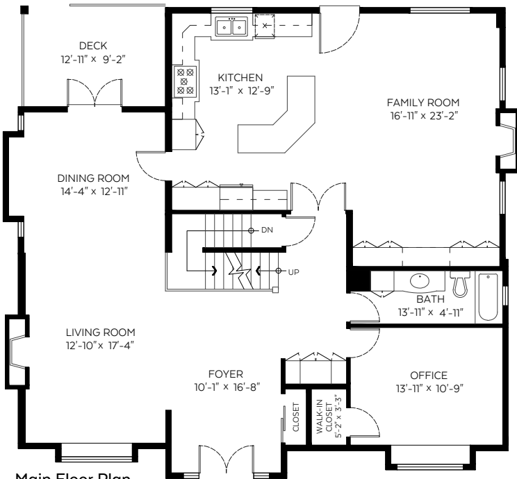
Main Floor Plan Floor Area: 1,720 sq.ft
