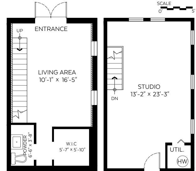
Studio-Lower Floor Plan Floor Area: 345 sq.ft Ceiling Height: 7'-6"
