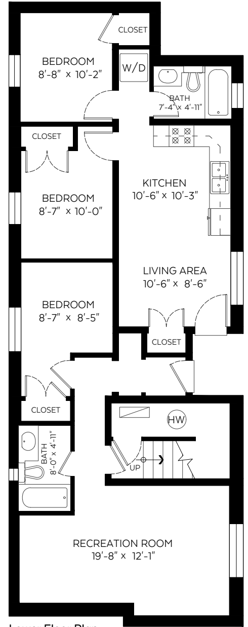
Lower Floor Plan Floor Area: 1,196 sq.ft
