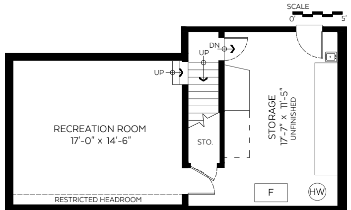
Lower Floor Plan Floor Area: 590 sq.ft
